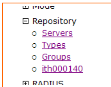
Figure 7. Repository menu
