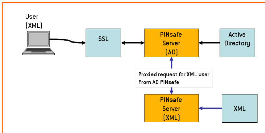
Figure 28.Example of peering fro multi-repository installation
