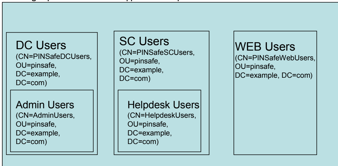
Figure 51.More complex repository groups example – AD structure
