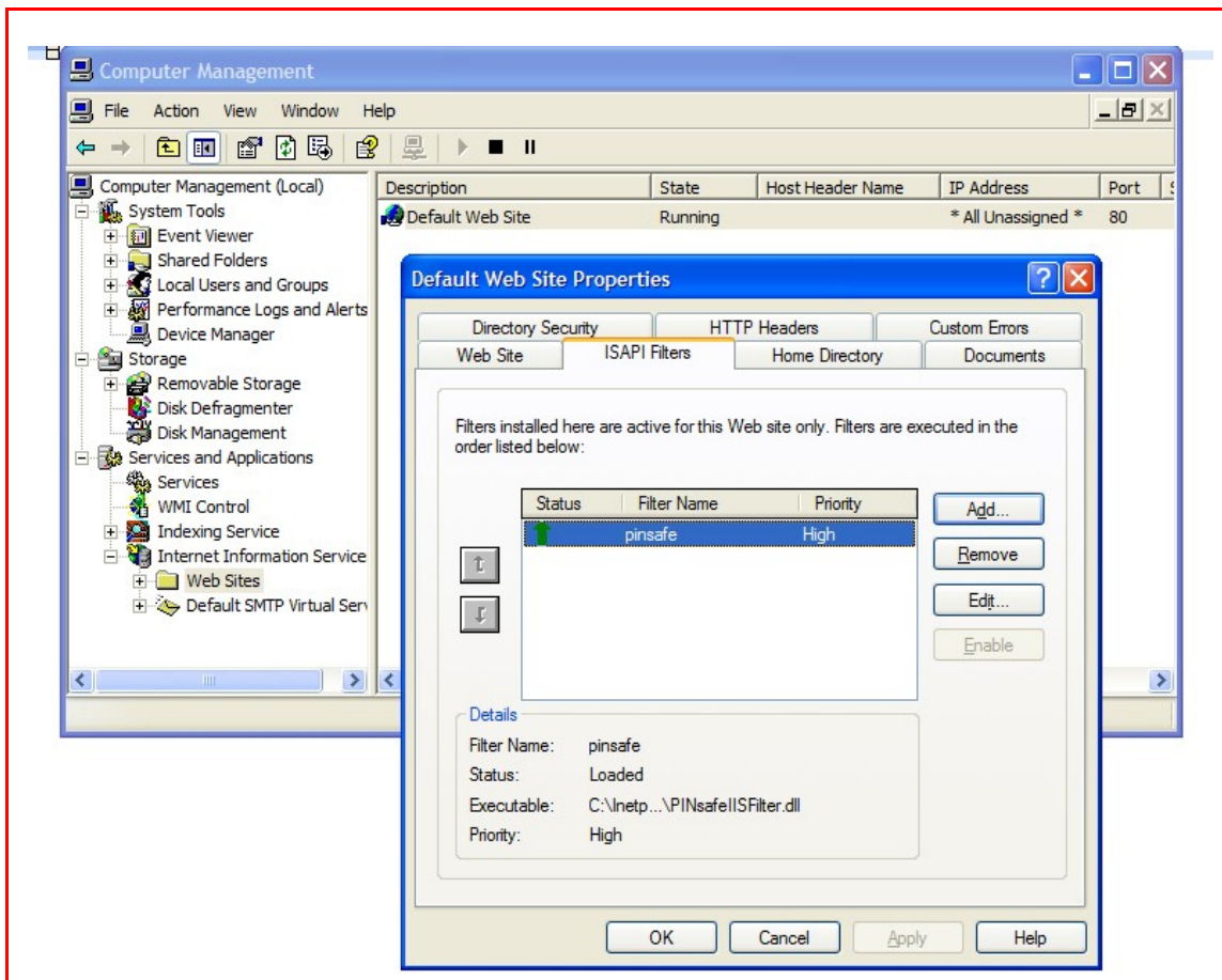
Figure 21.Screenshot of IIS filter installation
